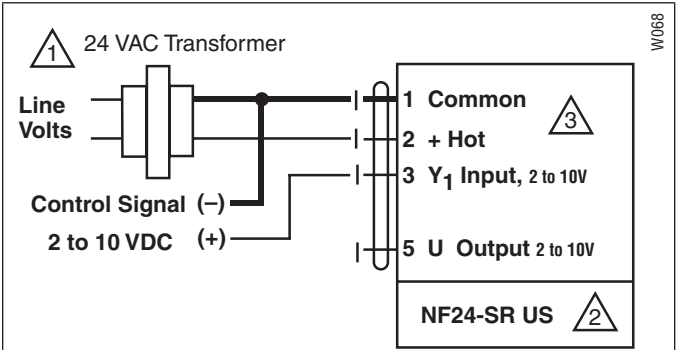
2 to 10 VDC control of NF24-SR US
