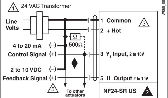
4 to 20 mA control of NF24-SR US with 2 to 10 VDC feedback output
