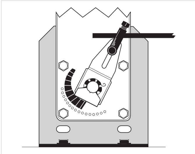
KH-AF non-direct mounting with ZG-108 mounting bracket
