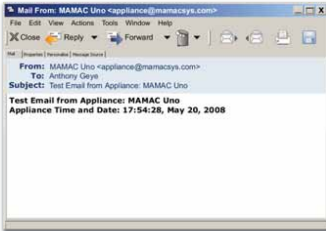
Test email
