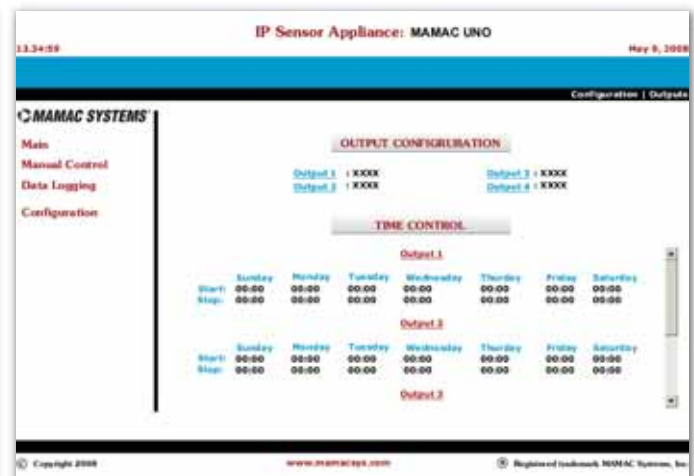
Output configuration
