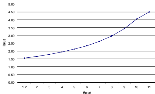
PS1X03 Safe Operating Range - 12Vac Input
