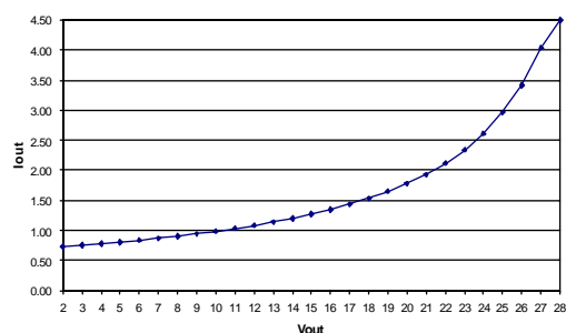
PS1X03 Safe Operating Range 24 Vac Input
