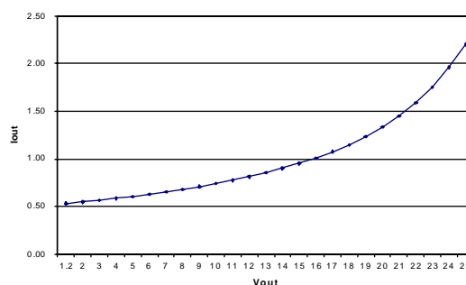
PS1X01 Safe Operating Range - 24 Vac Input
